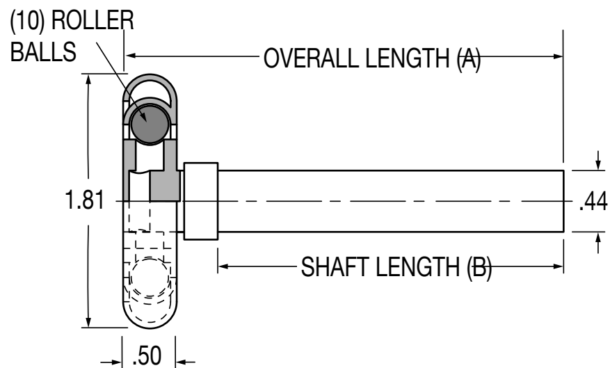
2" Style Roller
