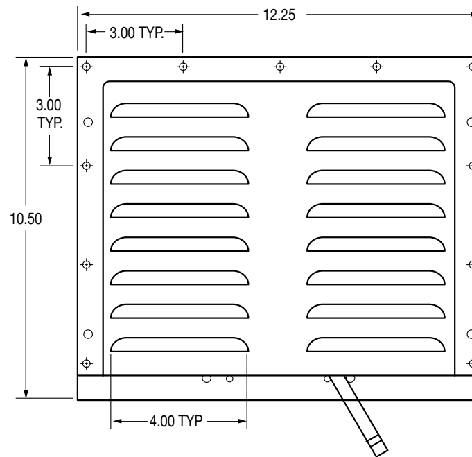
Adjustable Louvered Vent Shown
