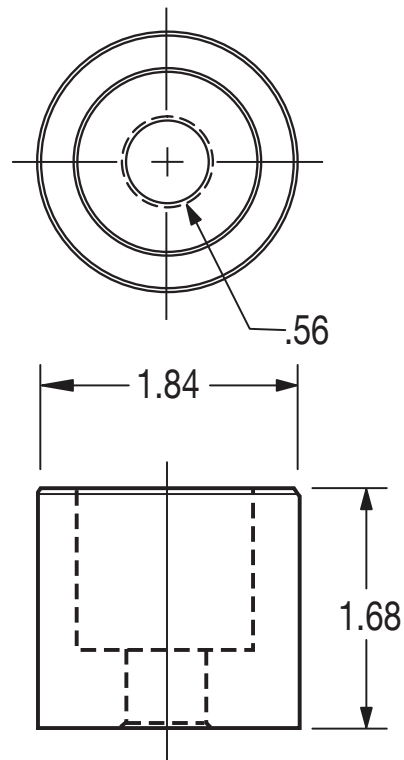
Utility Style Door Bumpers 022-01085
