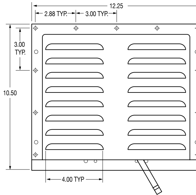
Adjustable Louvered Vent Shown
