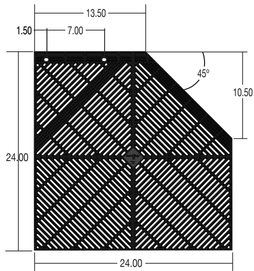
AeroFlap AF-24
